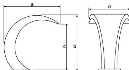
Vodní clona "BALI" "BALI" water curtain
