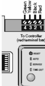
#75003 Digital Control Panel Base Plate
